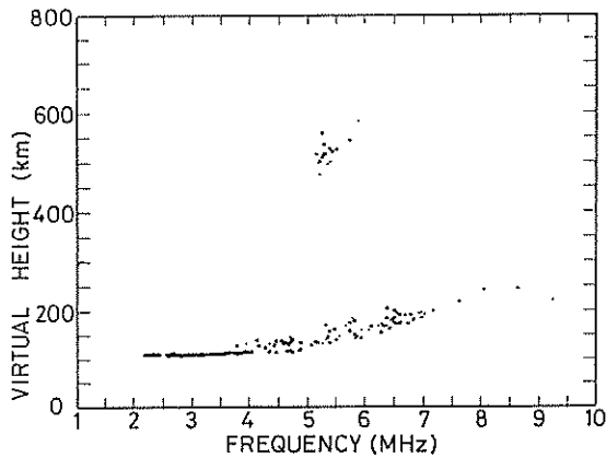
Fig. 3 Ionogram recorded at 1545 LT on 26 September 1982, showing normal E and F region traces together with a slant Es layer.
