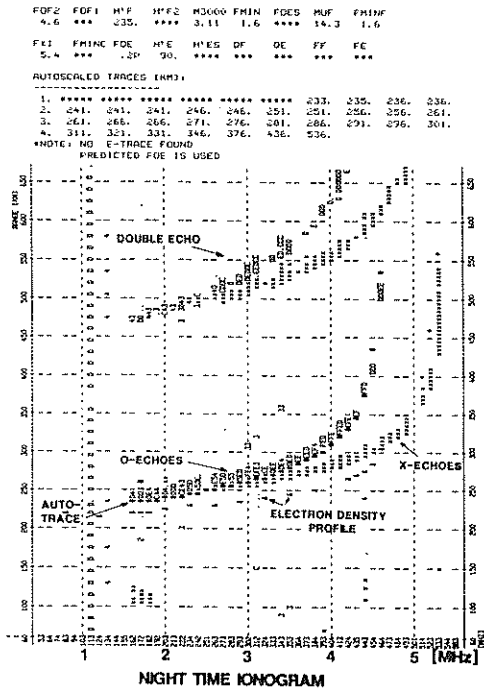
AUTO-SCALED TRACES AND ELECTRON DENSITY PROFILES ARE SUPERIMPOSED ON THE IONOGRAM. SCALED PARAMETERS ARE LISTED ON TOP.
