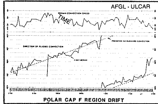
THE DIRECTION OF THE F REGION PLASMA DRIFT IN THE POLARCAP VARIES ALMOST LINEARLY WITH TIME, ROTATING 360° IN 24 HOURS. THE VELOCITIES VARY FROM 150 TO 750 m/s.
