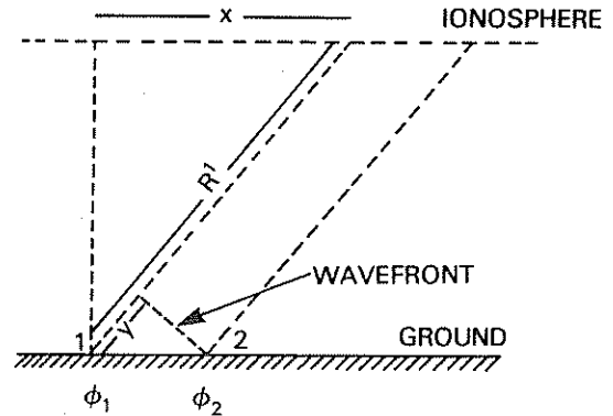
Fig. 2 Computation of the "skymap" position is determined by measuring the phase difference of the signals at antennas 1 and 2. y = (\phi_1 - \phi_2)\lambda / 2\pi , where \lambda is the wavelength of the sounding wave and x = y R^2 / d
