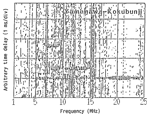
Fig. 2 An example of oblique ionogram obtained by using portable receiver with simple wire antenna.
